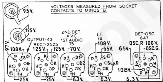
Fig. 1. Socket Voltage—Underside of Chassis View
